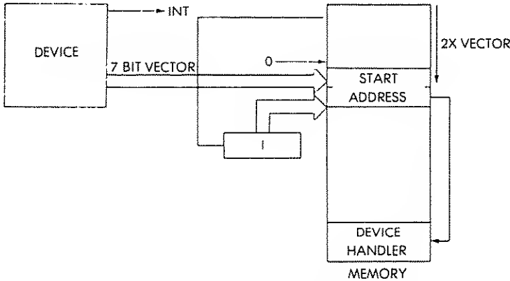
Fig. 6.29: Mode 2 Interrupt
