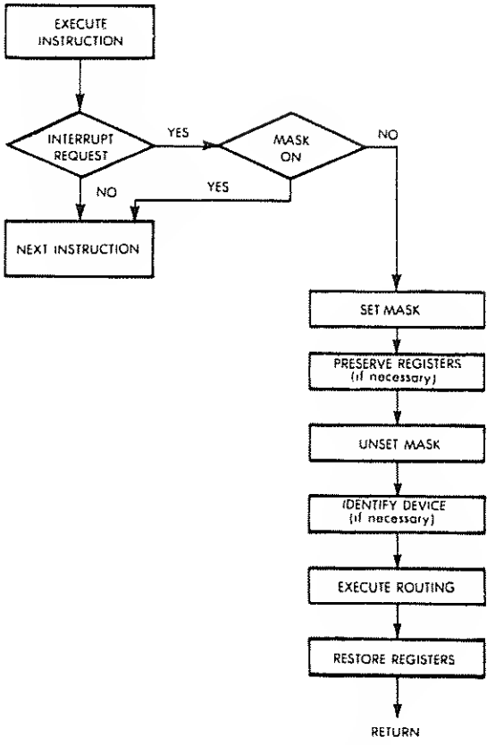
Fig. 6.34: Interrupt Logic
